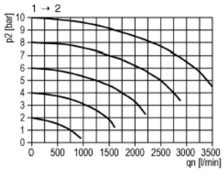
flow characteristic 1
