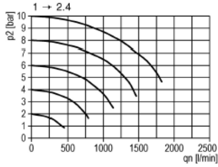
flow characteristic 2
